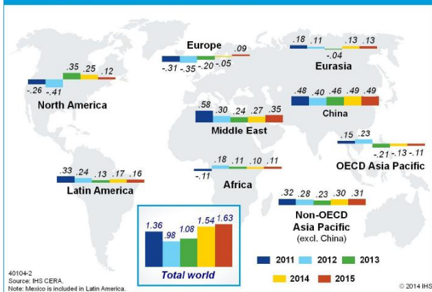
Changes in oil demand by region (volume change from previous year in million barrels per day)
